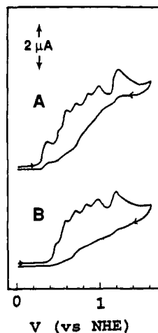
Figure 4. Cyclic voltammograms of \text{Ru}(\text{sar})^{2+} (A) and \text{Ru}(\text{imsar})^{2+} (B) in 0.1 M \text{CF}_3\text{SO}_3\text{H} on a glassy carbon electrode ( d = 0.6 \text{ cm} ) using a scan rate of 0.02 \text{ V s}^{-1} at 22 °C. [\text{Ru}^{\text{II}}] = 10^{-3} \text{ M} .
