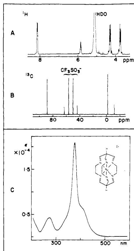
Figure 5. Upper part: 200 MHz ^1\text{H} and 50 MHz ^{13}\text{C} NMR spectra of \text{Ru}(\text{hexaimsar})^{2+} in \text{D}_2\text{O} (reaction mixture). Lower part: absorption spectrum of [\text{Ru}(\text{hexaimsar})](\text{PF}_6)_2 in \text{H}_2\text{O} .
