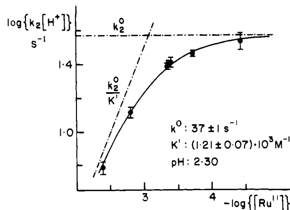
Figure 2. Dependence of the rate constant k_2 (eq 5) for the disproportionation of Ru(sar)^{3+} upon [H^+] and [Ru(sar)^{2+}] .
