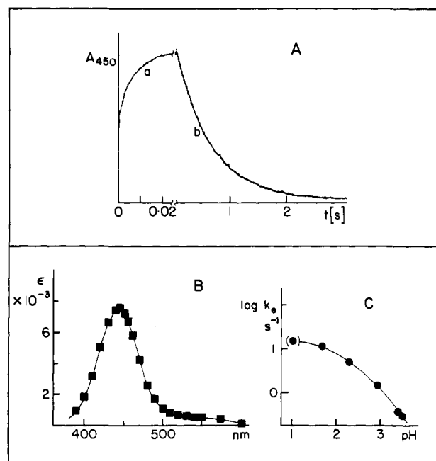
Figure 3. A: Transient absorption observed at 450 nm, ascribed to the deprotonated Ru^{IV}(sar-H^+)^{3+} complex, in reaction 20 (Table IV). B: Absorption spectrum for the Ru(IV) complex. C: Acid dependence of the Ru^{IV} \rightarrow Ru^{II} imine conversion ( k_e in Scheme II).
