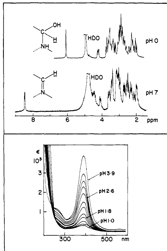
Figure 1. Upper part: 200 MHz ^1\text{H} NMR spectrum of \text{Ru}(\text{imsar})^{2+} in \sim 1 \text{ M DCl} (A, carbinolamine form) and in \text{D}_2\text{O} (B, imine form); lower part: \epsilon_{390} [\text{M}^{-1} \text{ cm}^{-1}] for \text{Ru}(\text{imsar})^{2+} as a function of pH.
